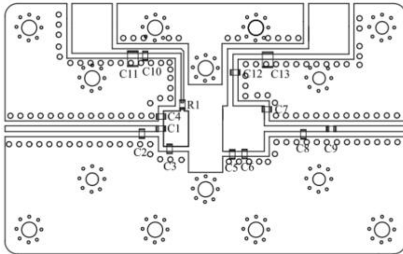
EVB Layout
